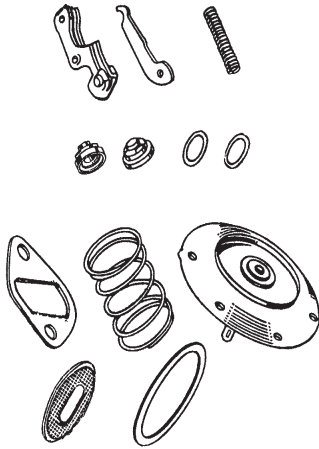
11A-9349 Fuel Pump Kit
